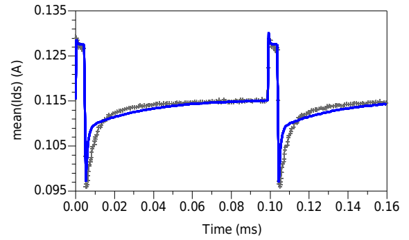
Fig. 4. Measurements (grey) and modeling (blue) of the average output current in pulsed RF signal operation at 10 GHz ( 5\mu\text{s} - 100\mu\text{s} ) with DC bias (20V, 115 mA). The amplitude of the transient induced by detrapping when RF is switched off is accurately modeled.
