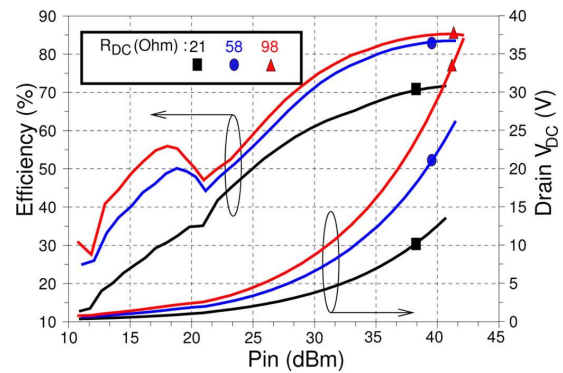
Fig.4. Conversion efficiency and drain dc output voltage versus input power for several dc drain resistor values. V_G =-4.4V and Z_{gate} = 230+j10Ω. The highest efficiency of 85% is obtained at 40dBm with a V_D =30V.
