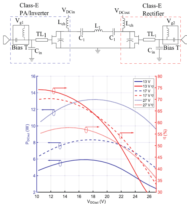
Fig. 7. Circuit diagram and measured total efficiency of class-E 2 self-synchronous dc-dc converter at 1.2GHz [3].
